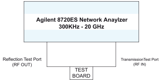
Figure #14. Test Setup
