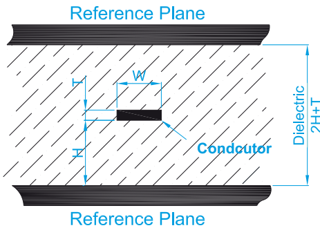
Figure # 13. Stripline geometry.
