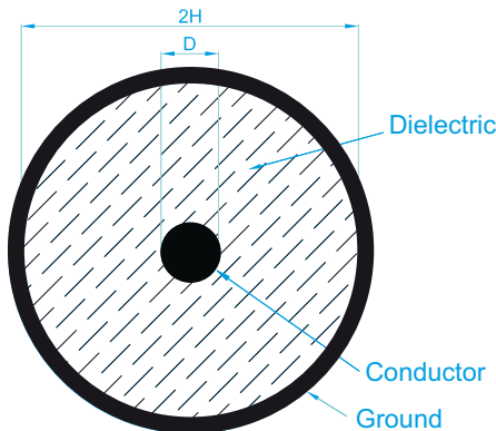
Figure # 10. Coaxial cable geometry
