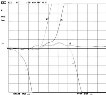
Figure # 24. Represents the characteristic impedance going through the Reed Relay shown in Figure # 9. Waves 1 through 5 depict calibration points. Horizontal full scale: 750 ps. Vertical scale: 150 milliUnit/div referenced from the 0 unit mark. The vertical scale measures the reflection coefficient.
