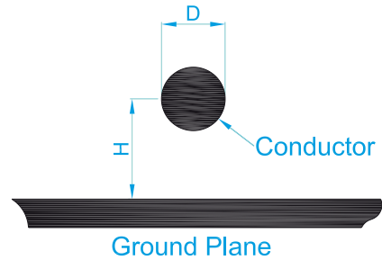
Figure # 11. Round wire over a ground geometry.
