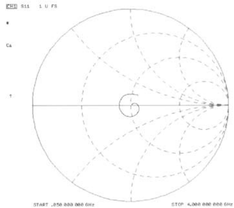
Figure # 25. Shows a Smith Chart plotted for frequencies to 4 GHz. The second dotted circle starting from the right is the 50 Ohm impedance point.
